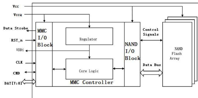
Figure3: eMMC architecture
